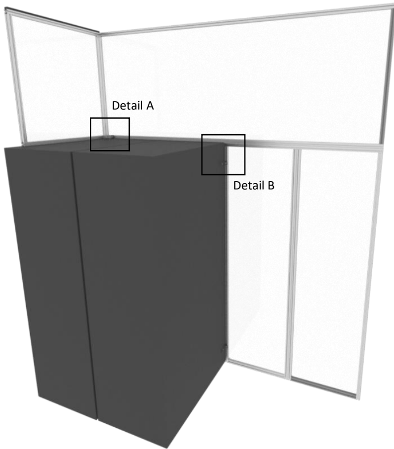
Mounting to the top of a cabinet
